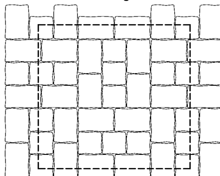
GRA-p08 * 17,36 ks/m 2 – granum 16/24 13,02 ks/m 2 – granum 16/16
