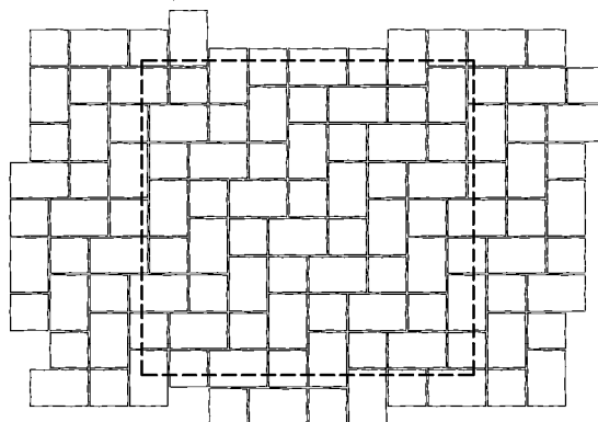
KOR-p08 27,78 ks/m 2 – korzo 12/12 27,78 ks/m 2 – korzo 12/18
