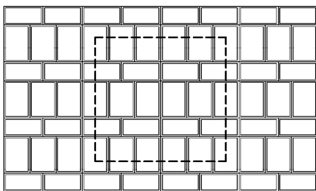
FOR-p07 7,41 ks/m 2 – forum 15/30 11,11 ks/m 2 – forum 20/30
