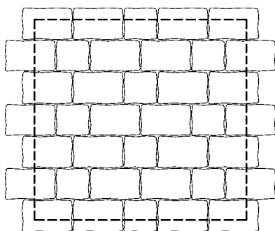
GRA-p05 * 19,53 ks/m 2 – granum 16/24 9,77 ks/m 2 – granum 16/16
