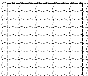
UNI-p01 39,51 ks/m 2 – normál
