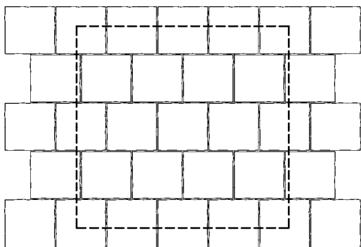
KOR-p07 27,78 ks/m 2 – korzo 12/12 27,78 ks/m 2 – korzo 12/18
