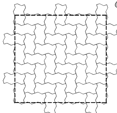
UNI-p06 26,34 (13,17) ks/m 2 – normál I (II)
