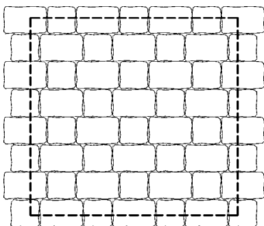
GRO-p03 20,41 ks/m 2 – graniko 14/21 20,41 ks/m 2 – graniko 14/14
