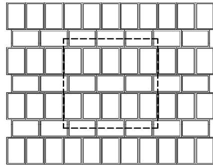
FOR-p08 13,33 ks/m 2 – forum 15/30 6,67 ks/m 2 – forum 20/30
