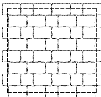
GRO-p05 25,51 ks/m 2 – graniko 14/21 12,76 ks/m 2 – graniko 14/14
