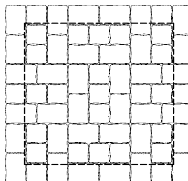
GRO-p08 22,67 ks/m 2 – graniko 14/21 17,01 ks/m 2 – graniko 14/14
