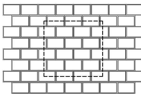
FOR-p02 16,67 ks/m 2 – forum 20/30
