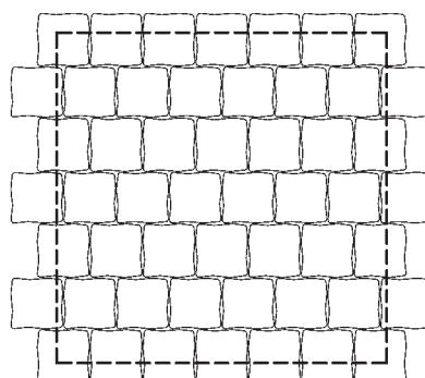
GRA-p06 * 15,63 ks/m 2 – granum 16/24 15,63 ks/m 2 – granum 16/16
