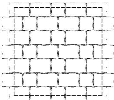
GRA-p05 * 19,53 ks/m 2 – granum 16/24 9,77 ks/m 2 – granum 16/16
